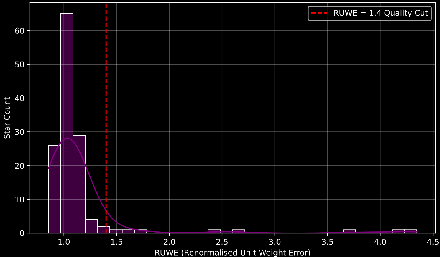
GAPOGEE DR17 Field [NGC7789_MGA] RUWE Distribution (n= 134)
