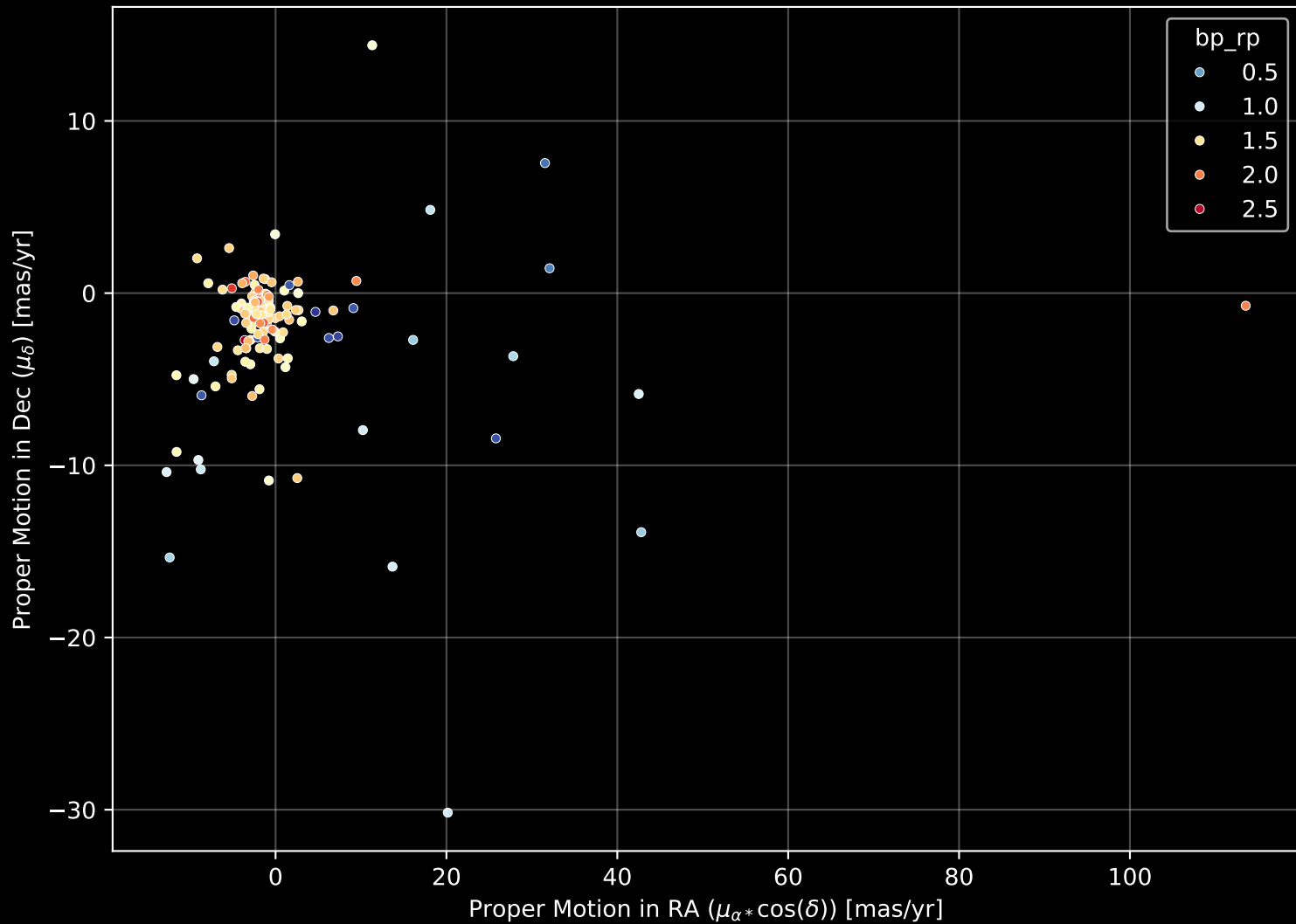
APOGEE DR17 Field: [NGC7789_MGA] Proper Motion Diagram (n= 137)
