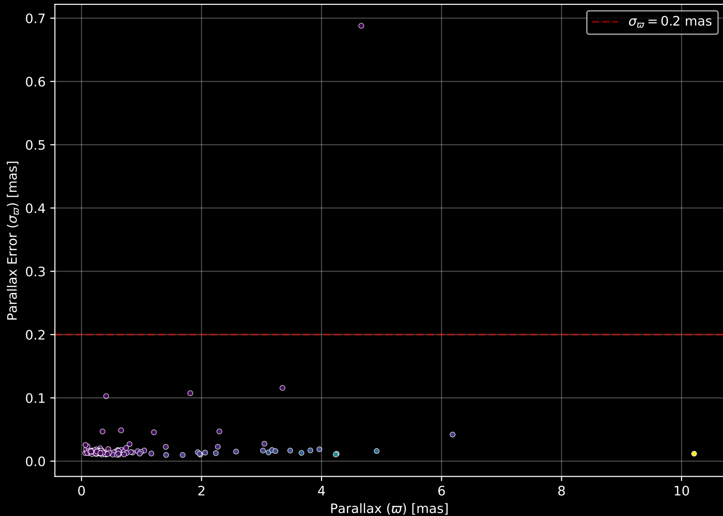
APOGEE DR17 Field: [NGC7789_MGA] Parallax Quality (n= 137)
