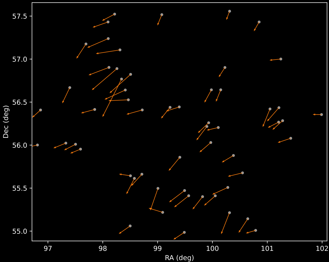
APOGEE DR17 Cluster 2 Proper Motion Vectors (n=56)
