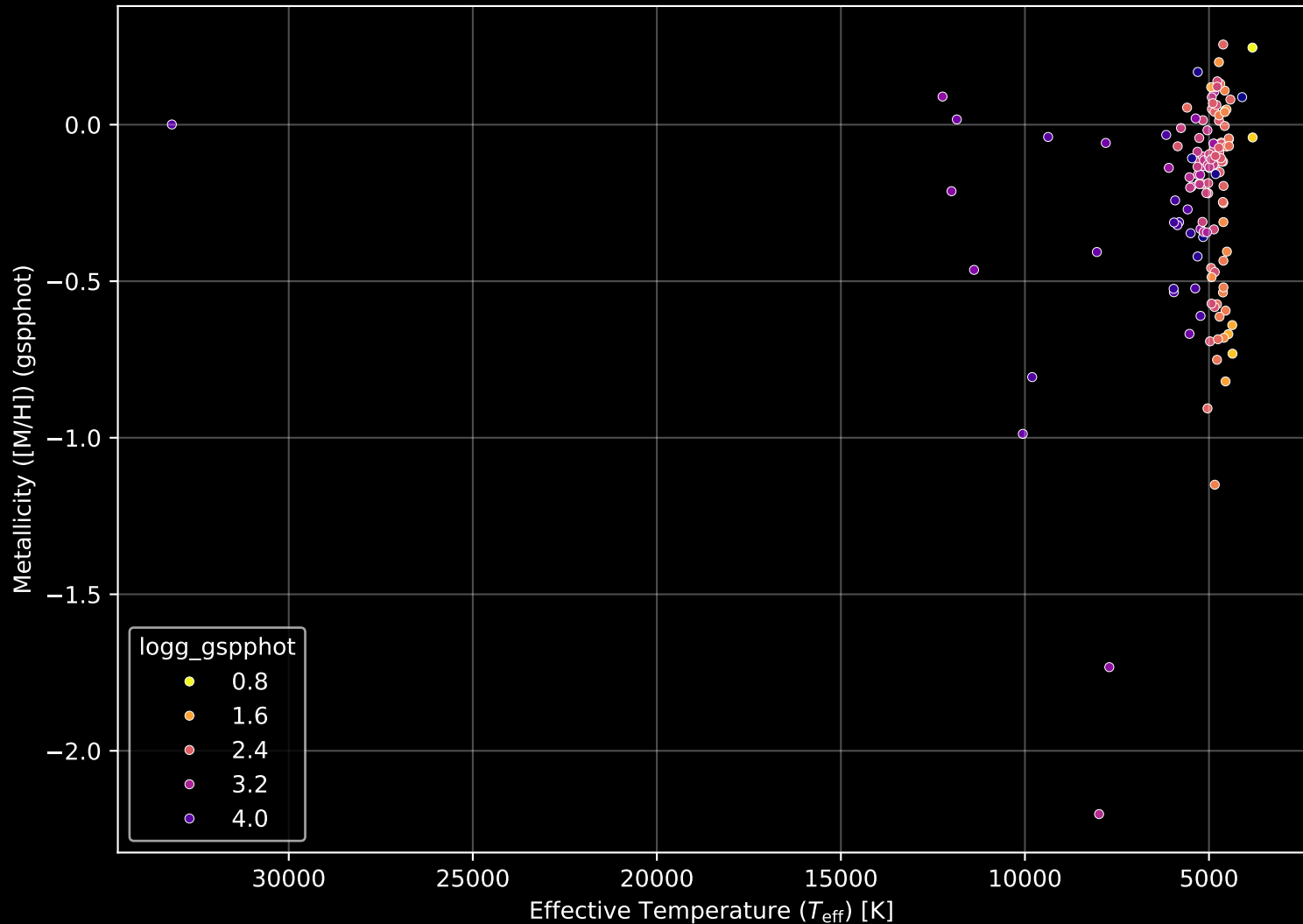
APOGEE DR17 Field: [NGC7789_MGA] Stellar Population Parameters (n= 137)
