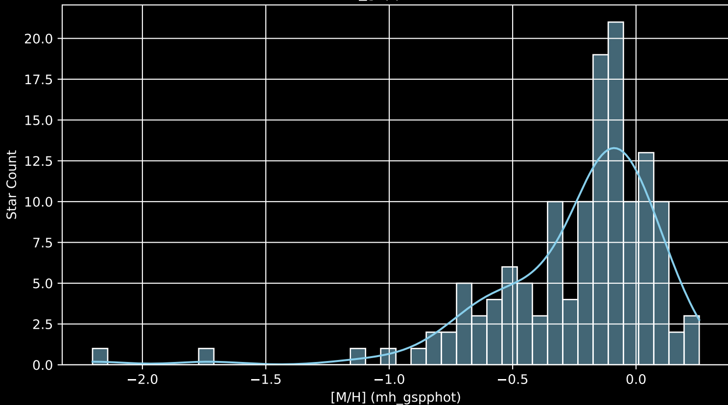
APOGEE DR17 Field: [NGC7789_MGA [M/H] (mh_gspphot) (n= 137)
