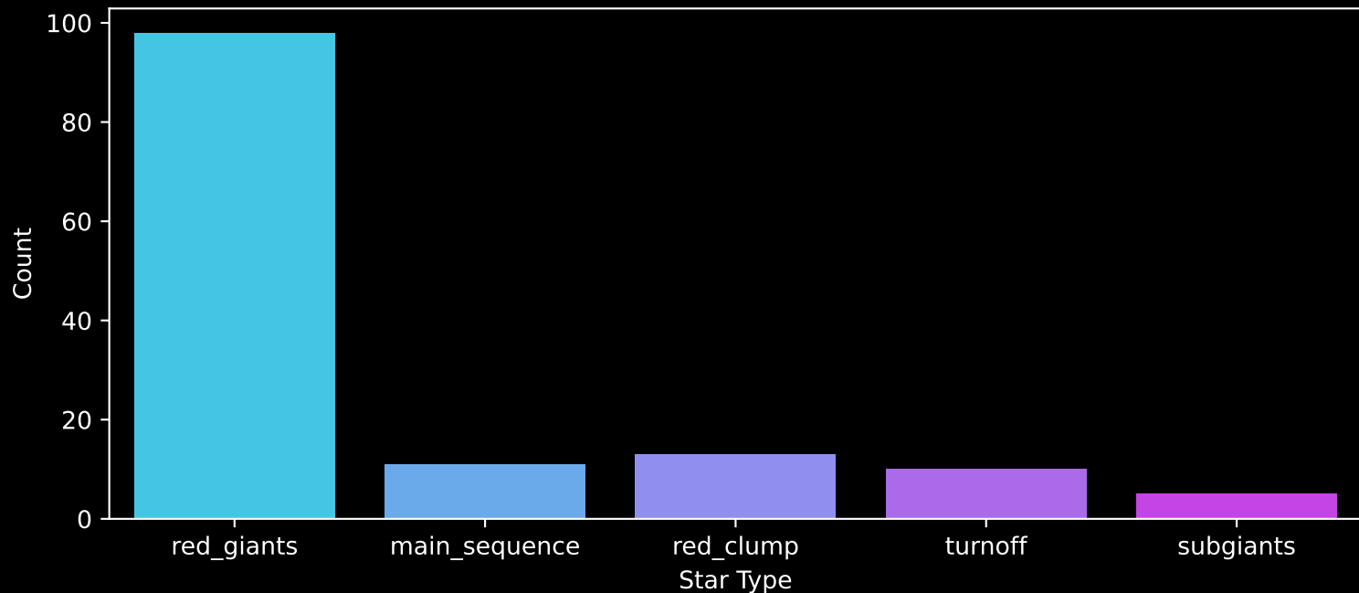
APOGEE DR17 Field: [NGC7789_MGA] Count plot of Star Type
